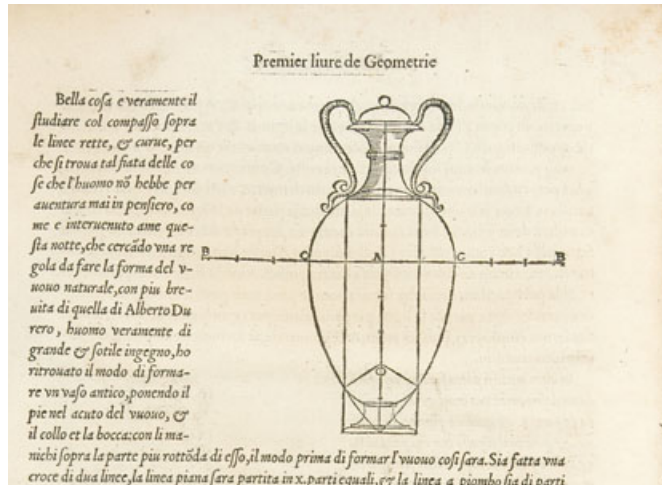
Both Dürer and Serlio introduce the principle of drawing arcs taking the ovum as an example. The construction begins with the divisions of an orthogonal frame. The radii measurements are based on the approximations of the harmonic section.
